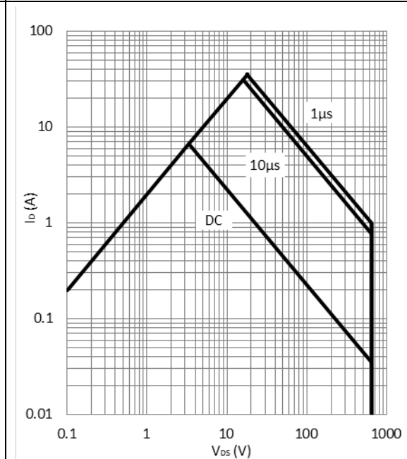
Figure 14. Safe Operating Area T_c=80^\circ\text{C}
