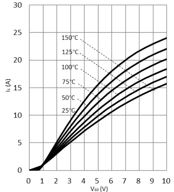
Figure 8. Forward Characteristic of Rev. Diode
