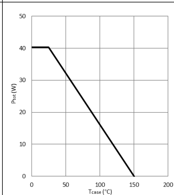
Figure 10. Power Dissipation
