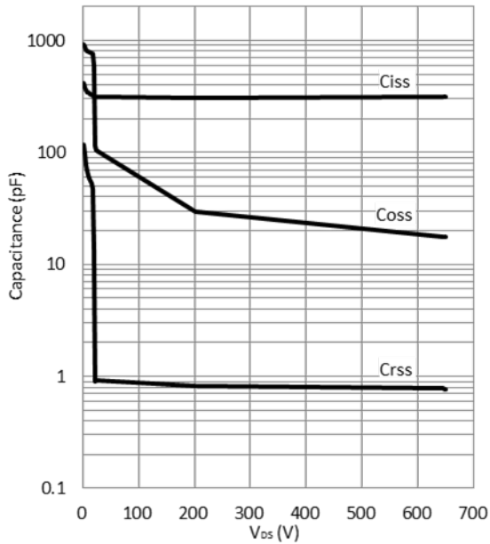
Figure 5. Typical Capacitance
